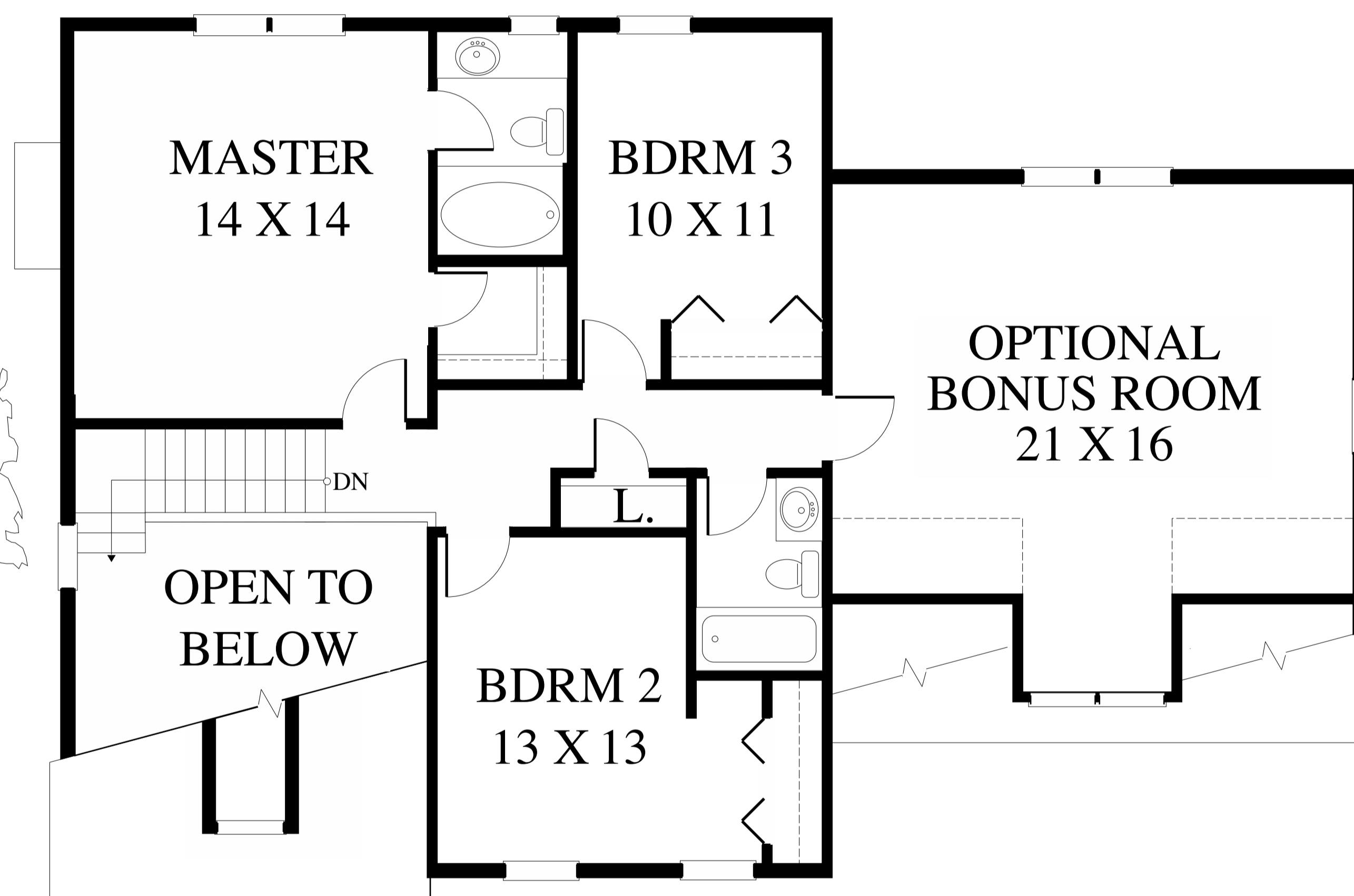
SECOND FLOOR
