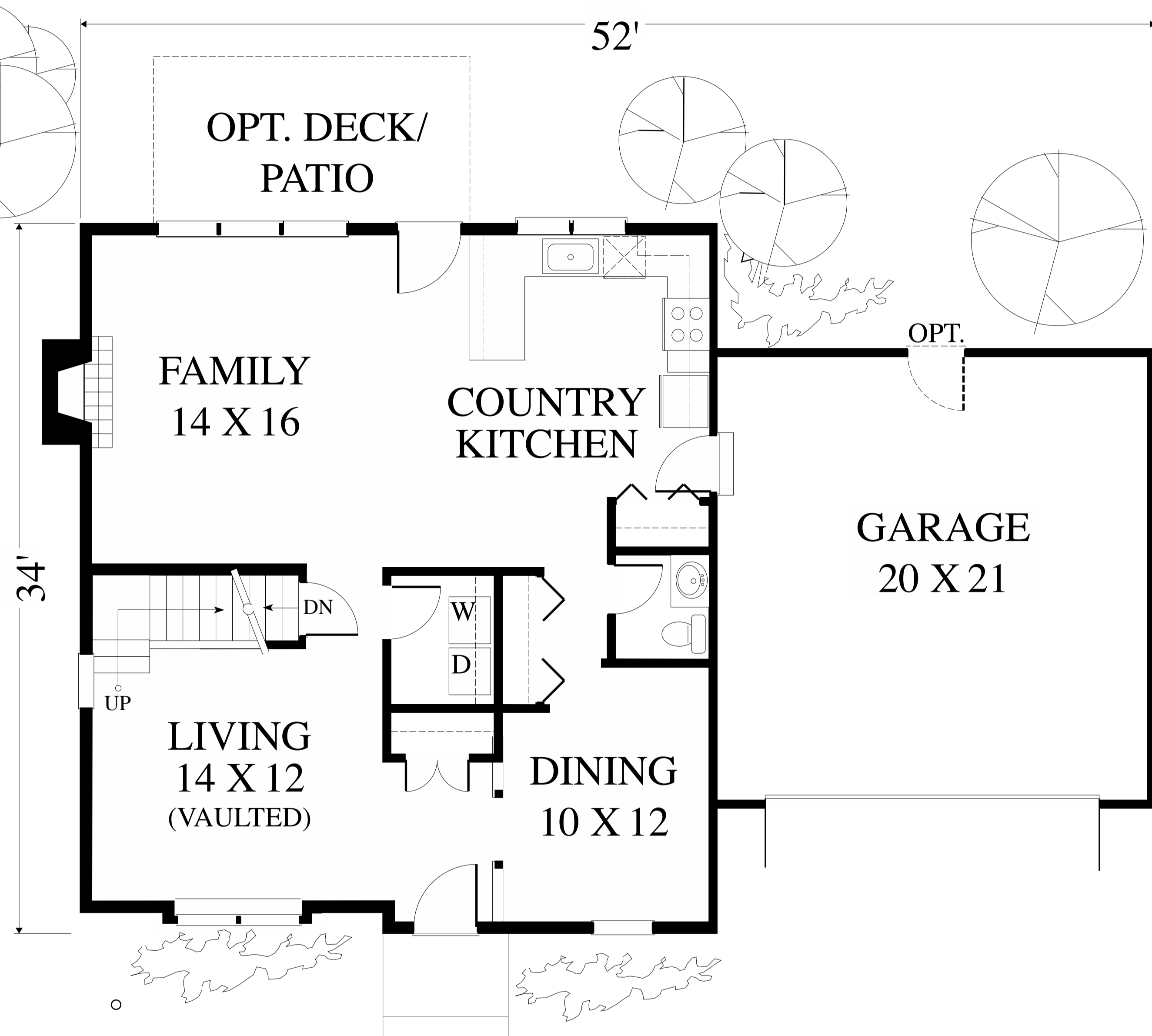
FIRST FLOOR
